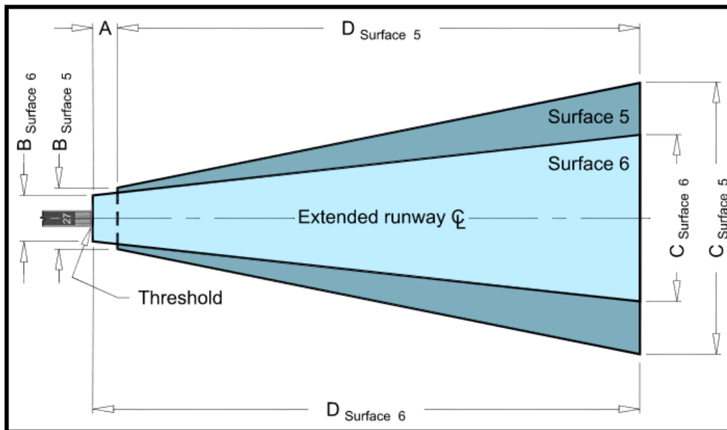
Figure 3-7. Approach Procedure with Vertical Guidance (APV) and Precision Approach (PA) Instrument Runway Approach Surfaces
